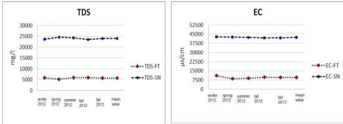
Figure 1. Variation of total dissolved minerals and water EC in Fotoyeh and Sangueyeh Springs
