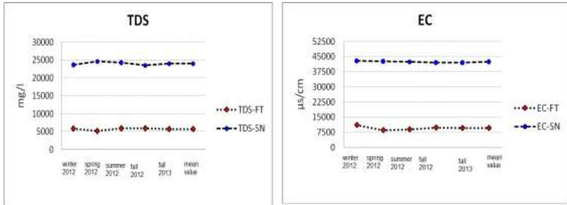
Figure 1. Variation of total dissolved minerals and water EC in Fotoyeh and Sangueh Springs
